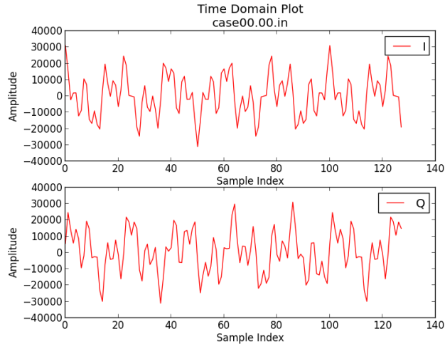
Figure 2: Time Domain Tones with Spectral Image
