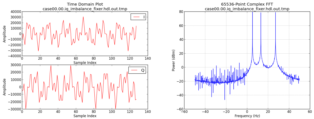
Figure 4: Time Domain Tones with Spectral Image re-moved re-Figure 5: Frequency Domain Tones with Spectral Image removed
