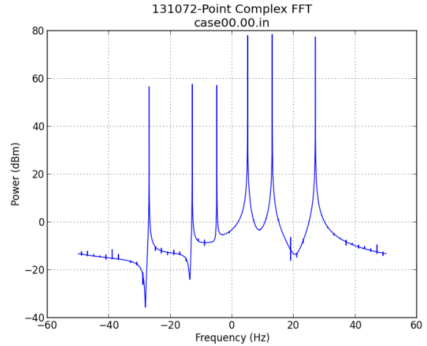
Figure 3: Frequency Domain Tones with Spectral Image
