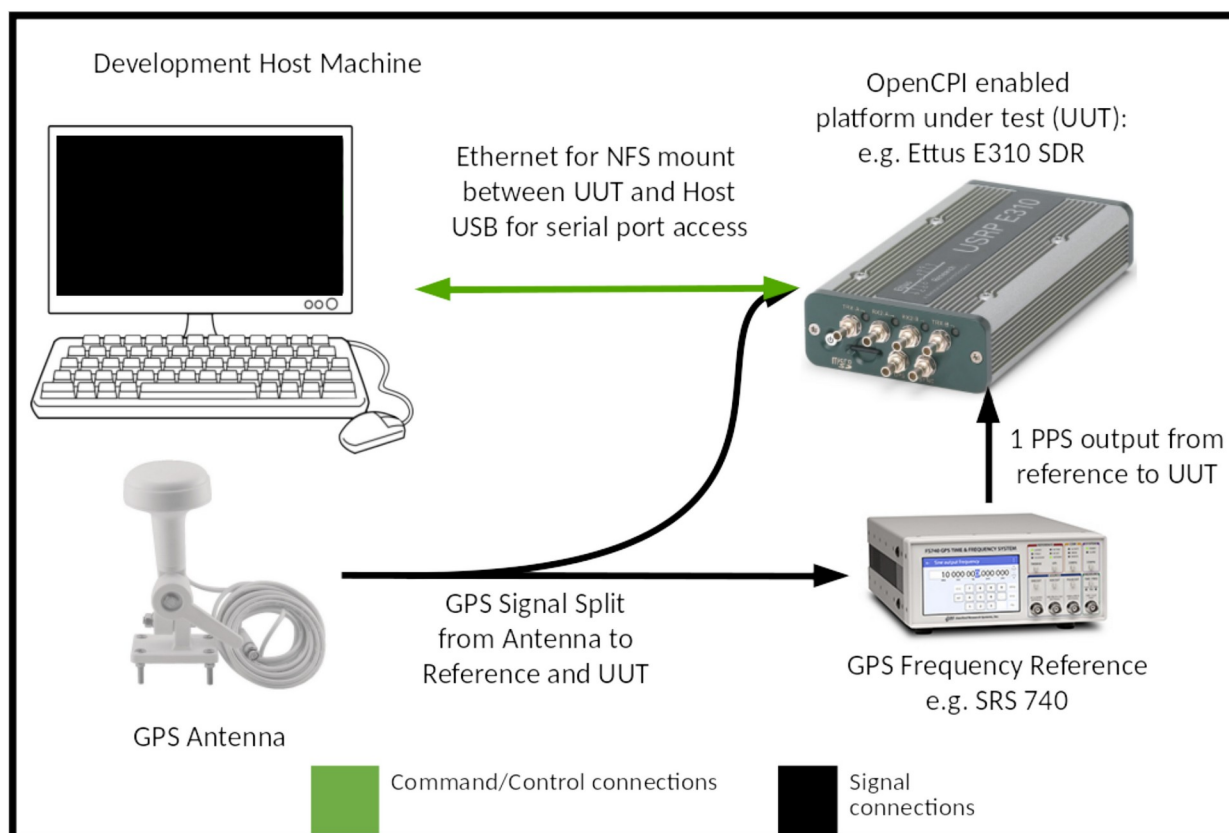
Figure 12: Timestamping Accuracy Measurement
