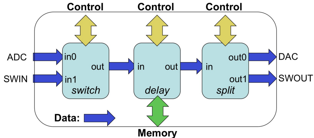
Figure 4: Example HDL Assembly
