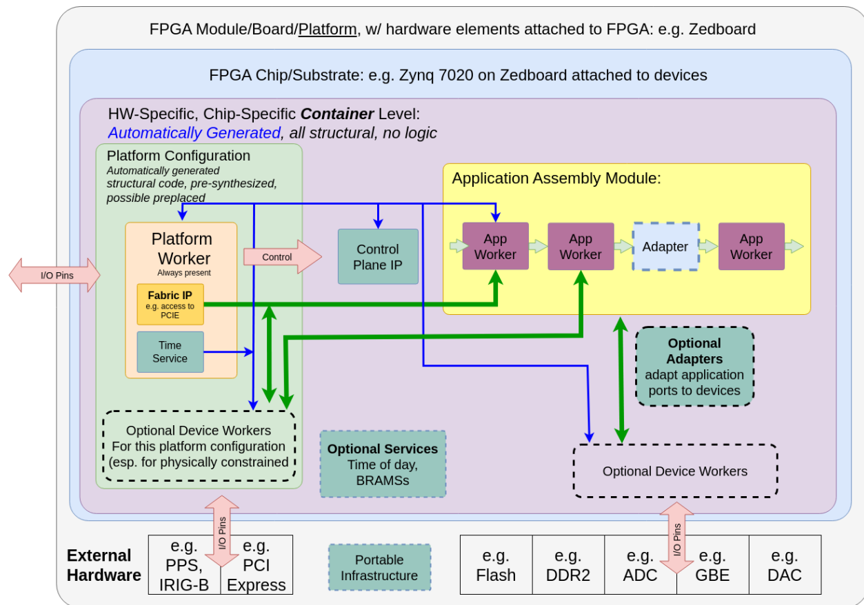
Figure 10: HDL Full FPGA Hierarchy
