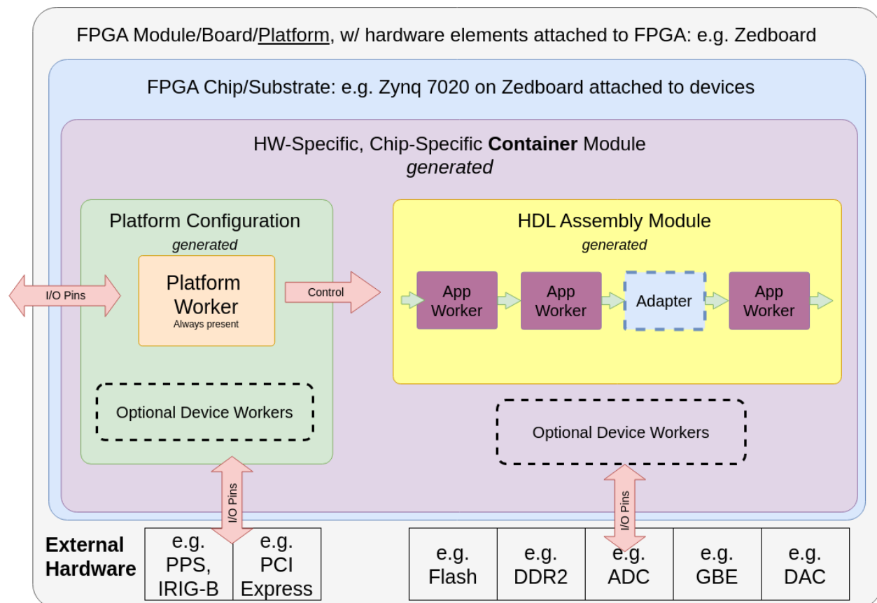
Figure 1: HDL Hierarchy
