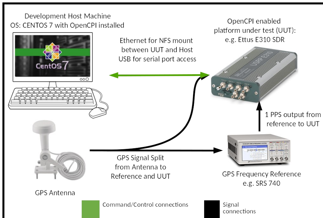
Figure 12: Timestamping Accuracy Measurement
