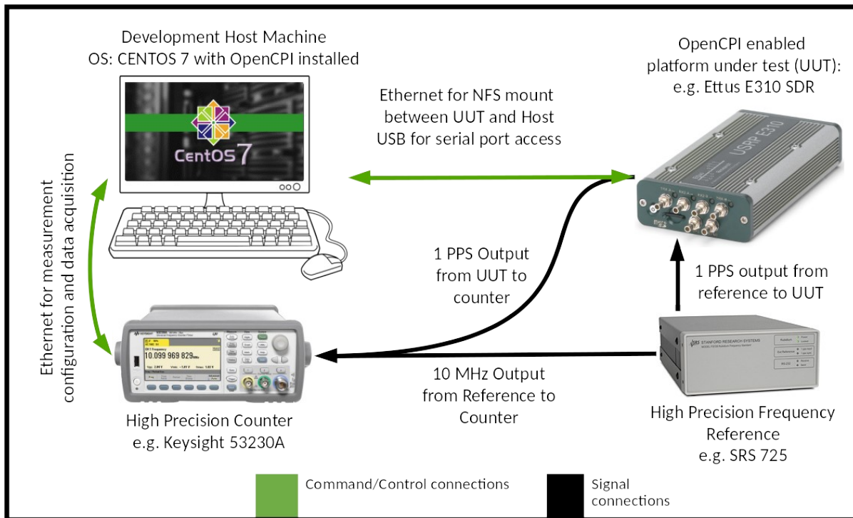
Figure 11: Timekeeping Clock Measurement Setup
