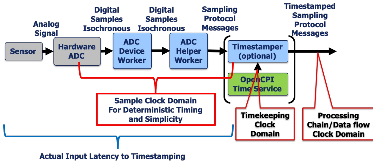
Figure 10: ADC Device Support Model
