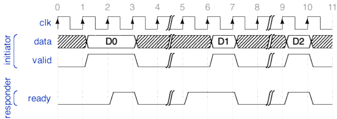
Figure 3: Three SDP Transfers with Different Ready and Valid Assertions
