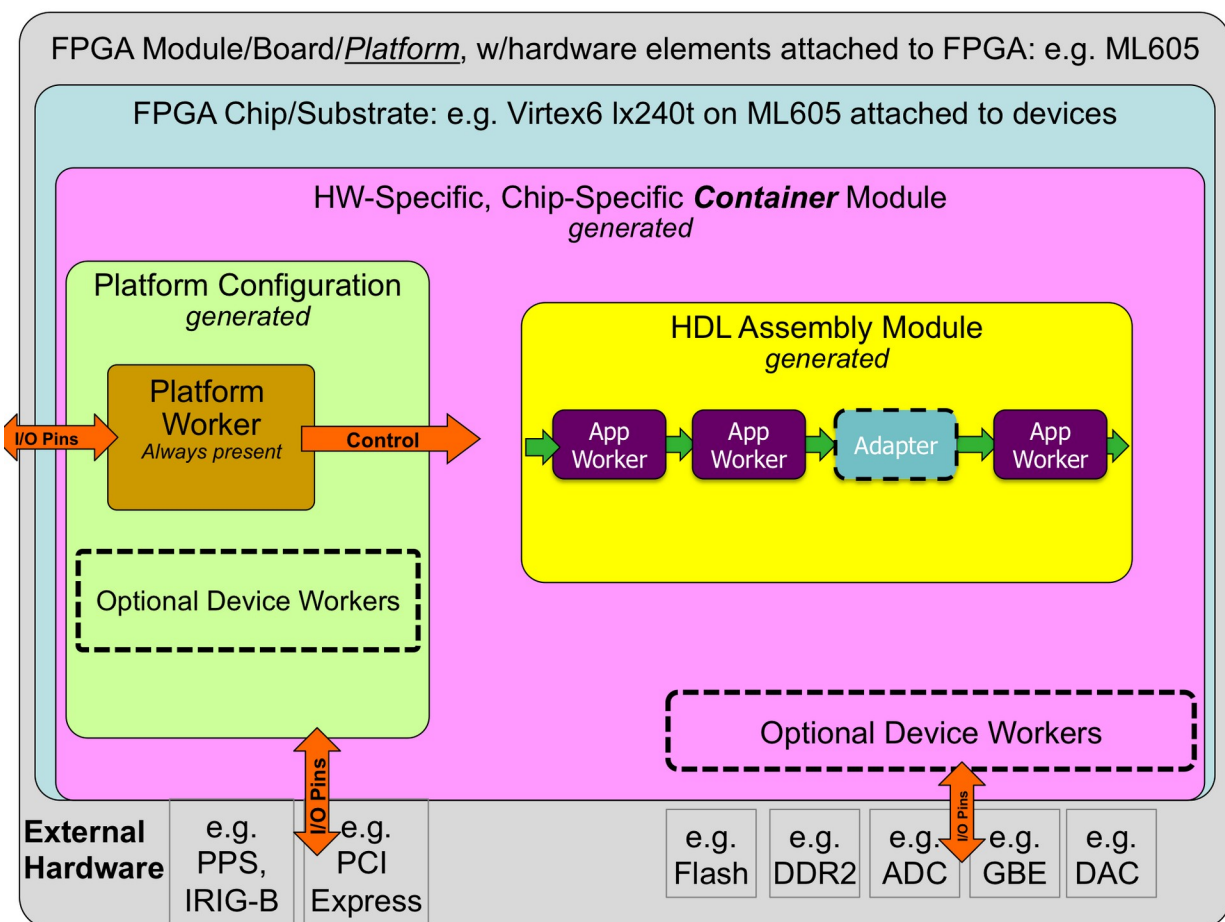
Figure 1: HDL Hierarchy
