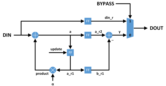
Figure 2: Circuit Diagram
