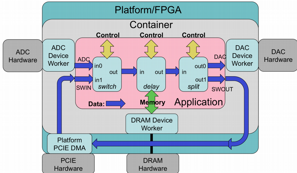
Figure 6: OpenCPI HDL Assembly on Container and Platform
