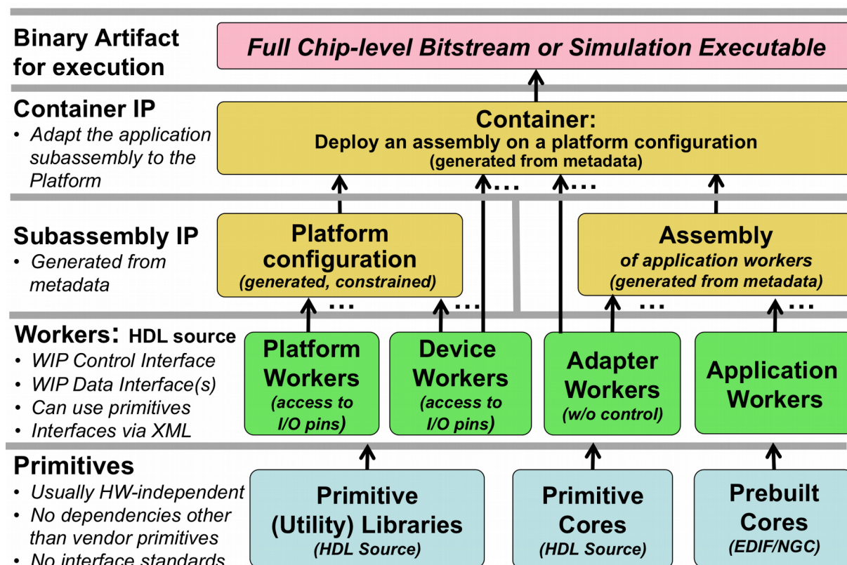
Figure 9: OpenCPI HDL Build Flow Layers
