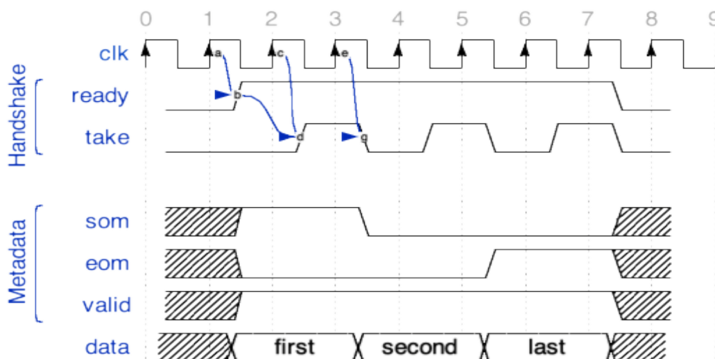
Figure 7: 3 word input message width worker adding delay
