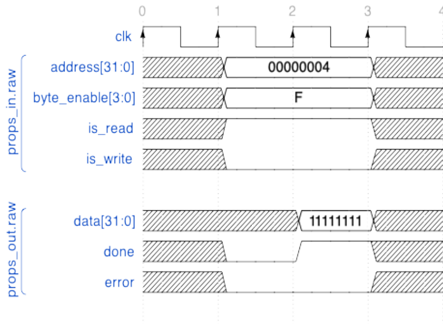
Figure 5: Raw Property Read of 32-bit Property
