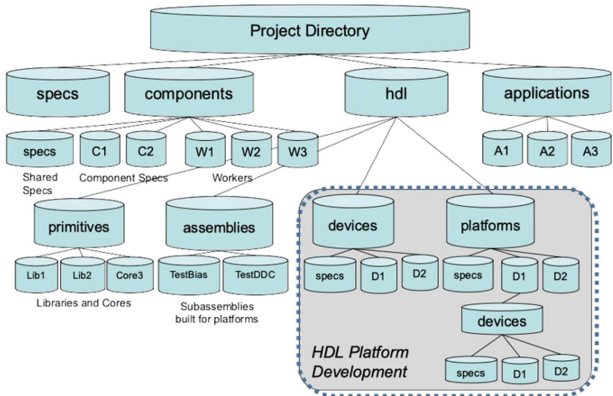
Figure 11: OpenCPI HDL Directory Structure
