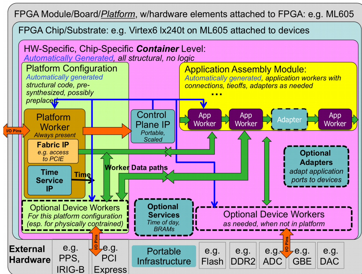
Figure 10: HDL Full FPGA Hierarchy
