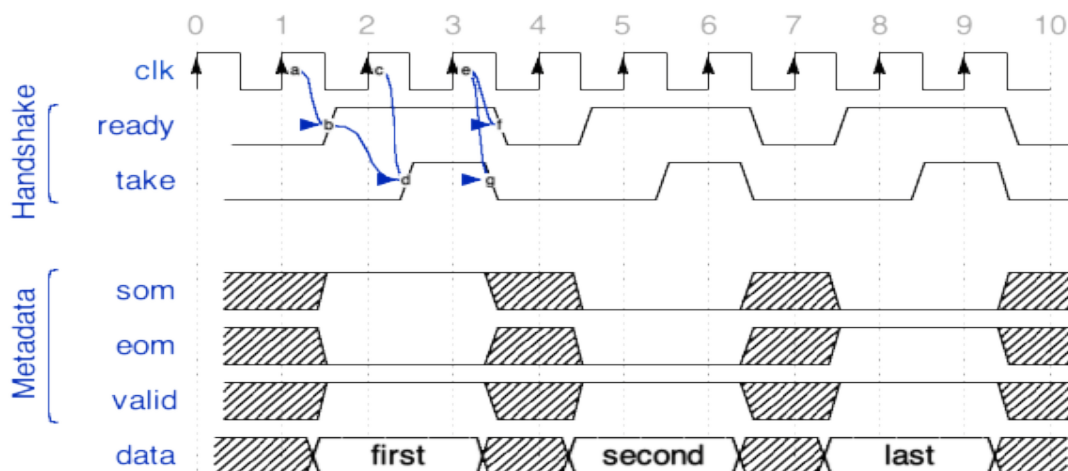
Figure 6: 3 word input message with delays on both sides
