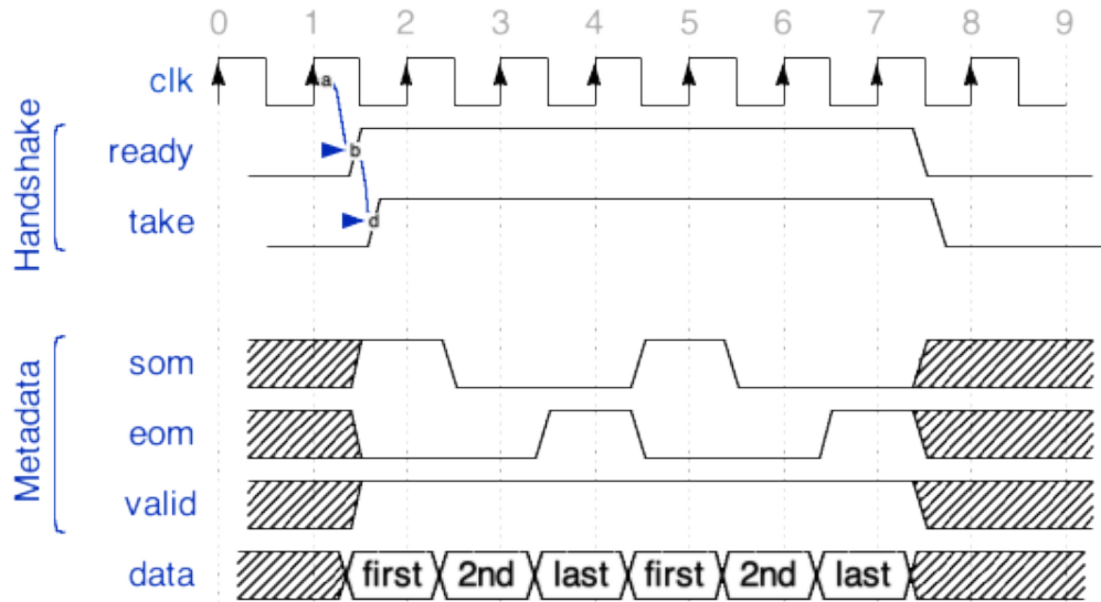
Figure 8: Two 3 word messages, with no delays on either side.
