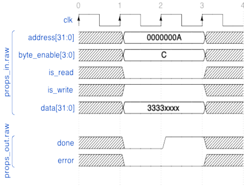
Figure 4: Raw Property Write to 16-bit Property
