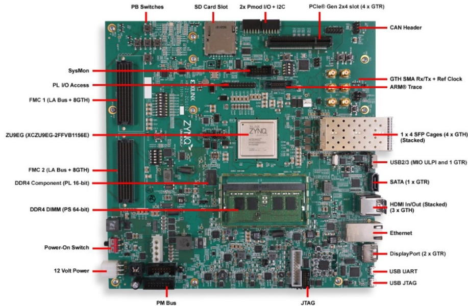
Figure 1: Xilinx ZCU102 Board Layout
