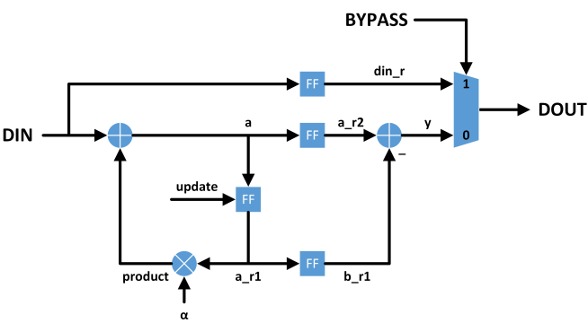
Figure 2: Circuit Diagram
