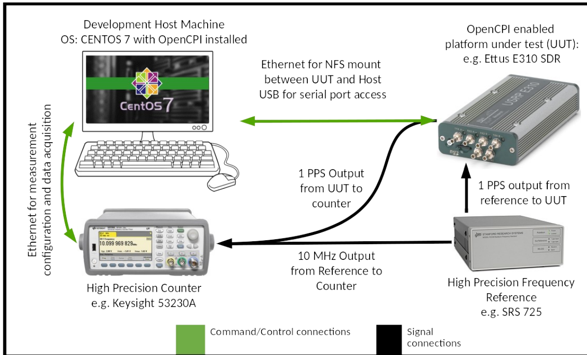
Figure 11: Timekeeping Clock Measurement Setup
