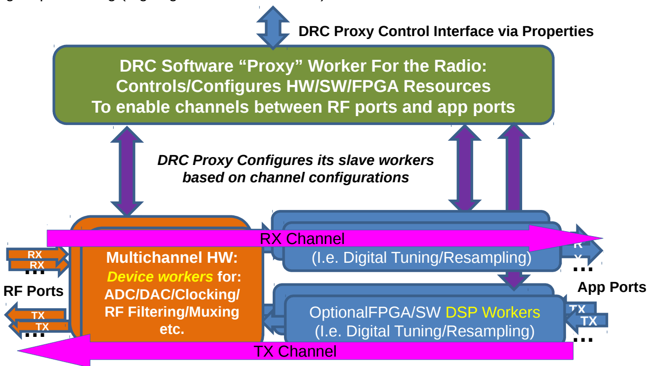
Figure 2: Digital Radio Controller Concept
